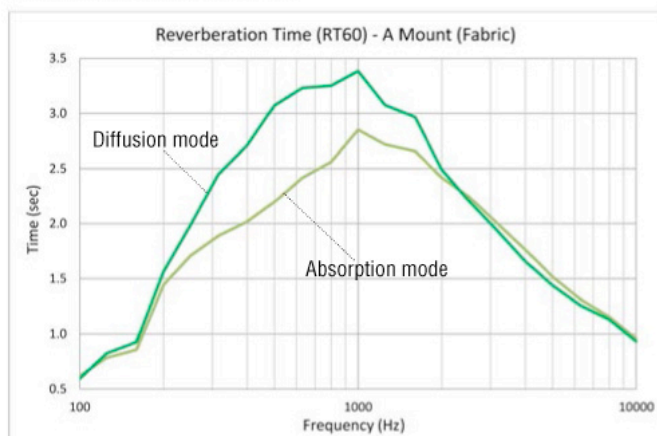
Two 4' x 4' panels stacked in reverberation room
